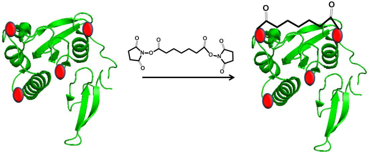
Figure 1-7: A schematic depiction of a crosslinking reaction, with Lysine residues shown in red.
