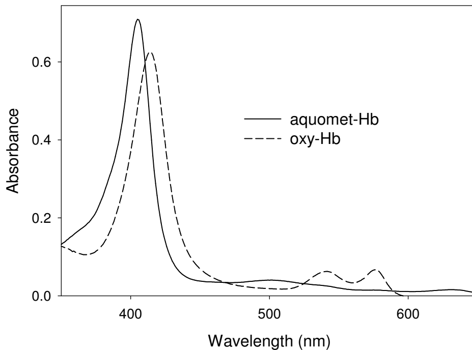
Figure 2-2: UV-Vis absorption spectra of oxy-Hb and aquomet-Hb in 10 mM ammonium acetate. The protein concentration was 3 \mu\text{M} for both samples. Differences in the intensity of the Soret peak are caused by the different molar absorption coefficients of the two forms 7 .
