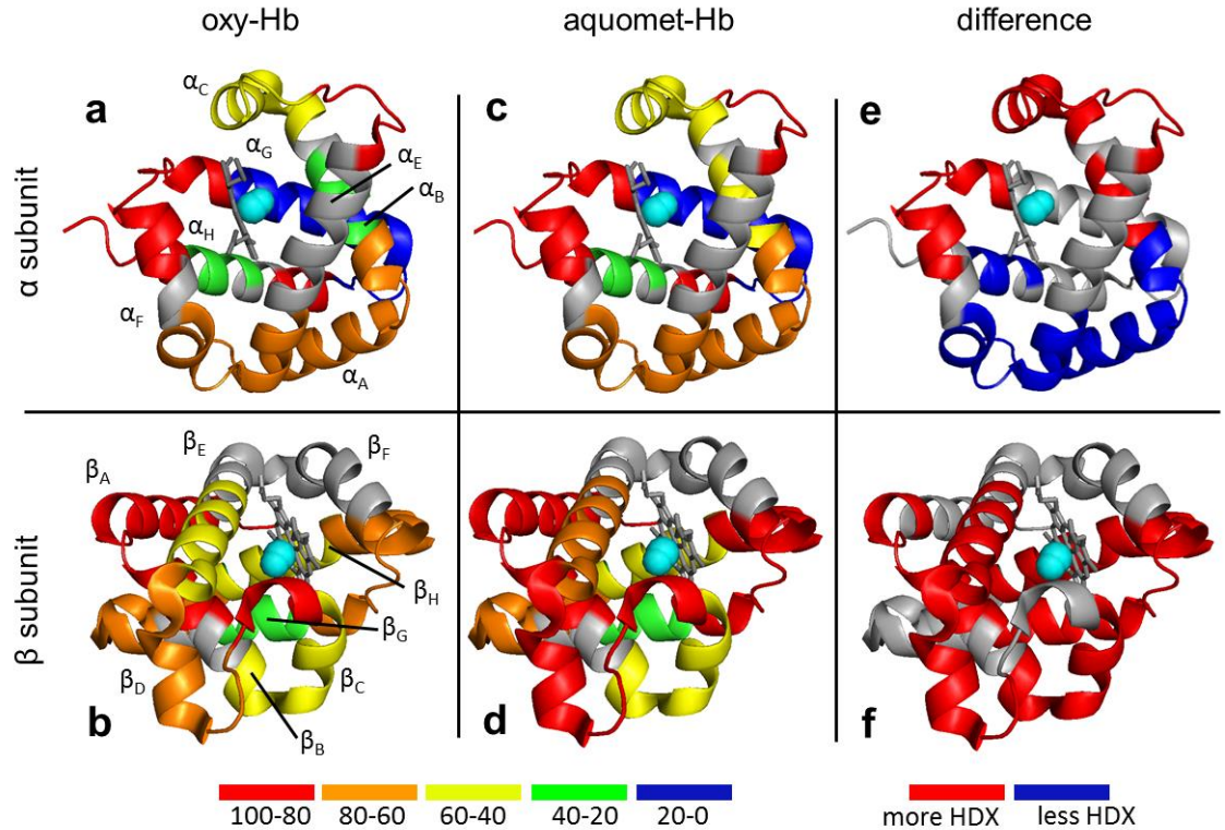
Figure 2-6: Mapping the HDX data of Figure 2-5 to the X-ray structure of bovine Hb 8 for t = 120 min. Using the orientation of Figure 2.1 as reference, the top row of panels in this Figure corresponds to \alpha 1 , the bottom row represents \beta 2 . Colors in (a) - (d) represent deuteration percentages, as defined in the legend along the bottom. Gray elements in (a) - (d) were not covered by peptide mapping. Panels (e), (f): Deuteration differences, calculated as [aquomet - oxy] for t = 120 min. Colored regions correspond to |difference| > 5\% . Segments that show elevated deuteration after oxy \rightarrow aquomet conversion are depicted in red. Segments with reduced deuteration are shown in blue. In all six panels the ligand binding site on the heme is highlighted in cyan.
