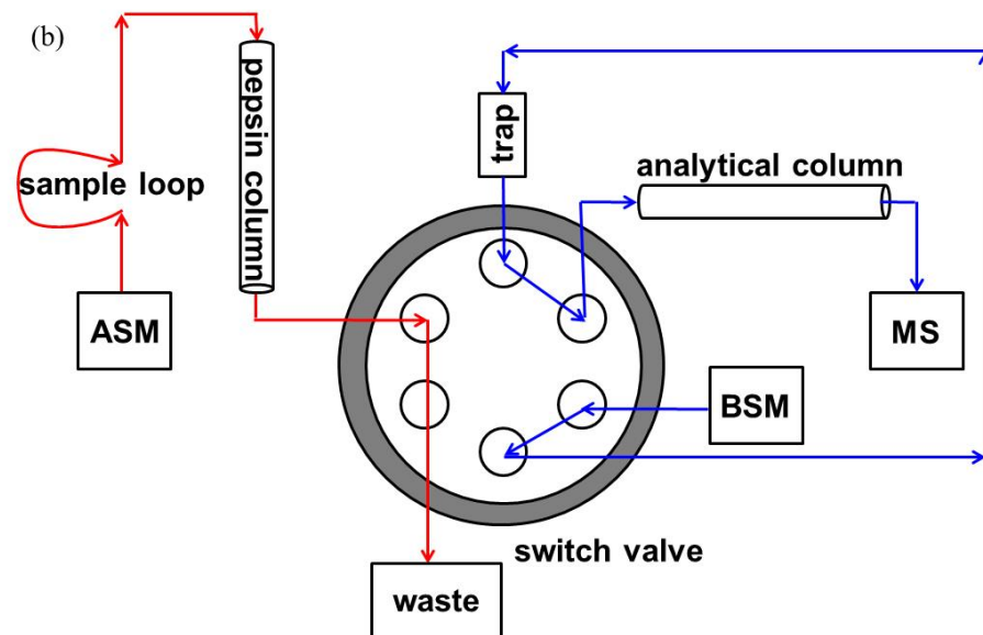
Figure 1-2: Layout of a typical fluidics unit for “bottom-up” proteolytic digestion HDX/MS experiments. (A) Isocratic flow (red) delivered by an auxiliary solvent module (ASM) moves the protein from the sample loop to a pepsin column for digestion. The resulting peptides are retained on a short trapping column. (B) Switching of the six-port valve allows the
